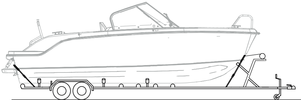
Figure 12.1 Cross 55 BR - Transport sur remorque
